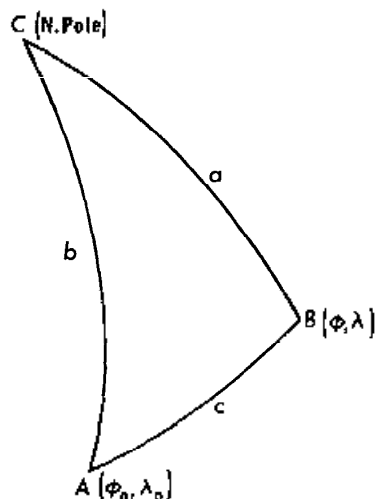
FIGURE 5.—Spherical triangle.
